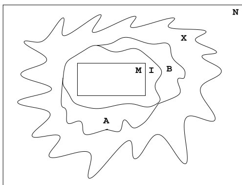
Figure 5.1: M \subset I \subset A, B \subset X \subset \mathbb{N}
